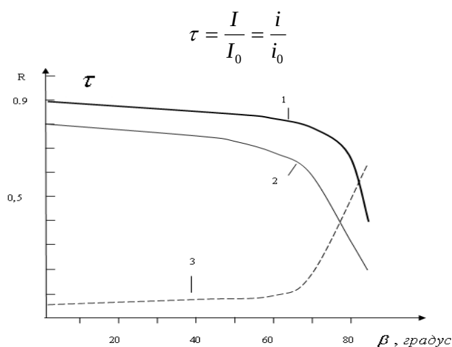
Рasm.2. Shaffof izolyatsiya yorug'lik o'tkazish koefitsientining ( \tau ) nurning tushish burchagiga bog'liqligi.
