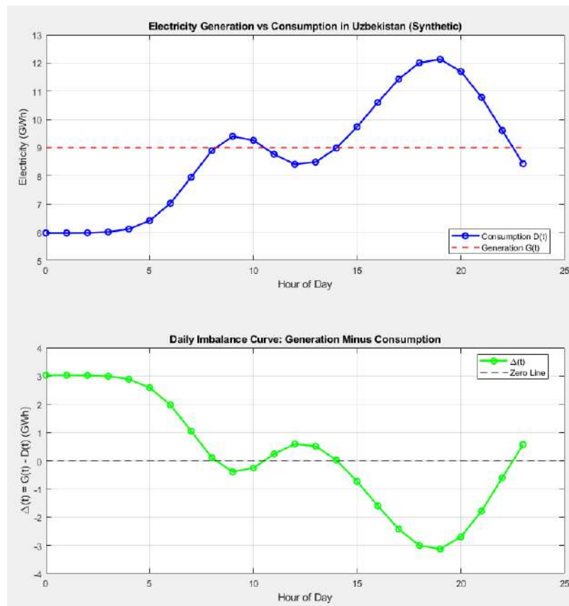
Figure 1. Daily Power Consumption and Generation Imbalance
