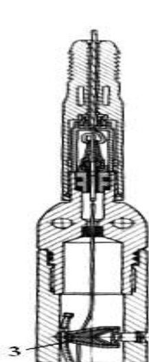
1-rasm. PK105DU korpusli kumulyativ perforatorining qurilmasi:
