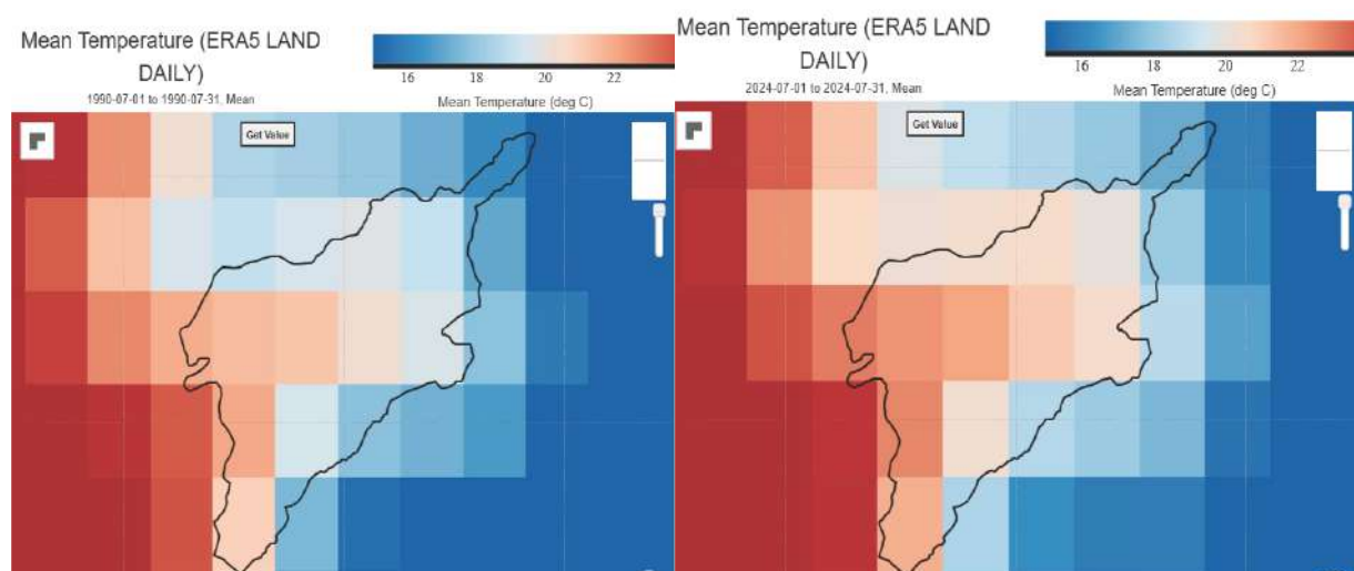
Figure 3. Temperature change maps generated using Climate Engine for July
