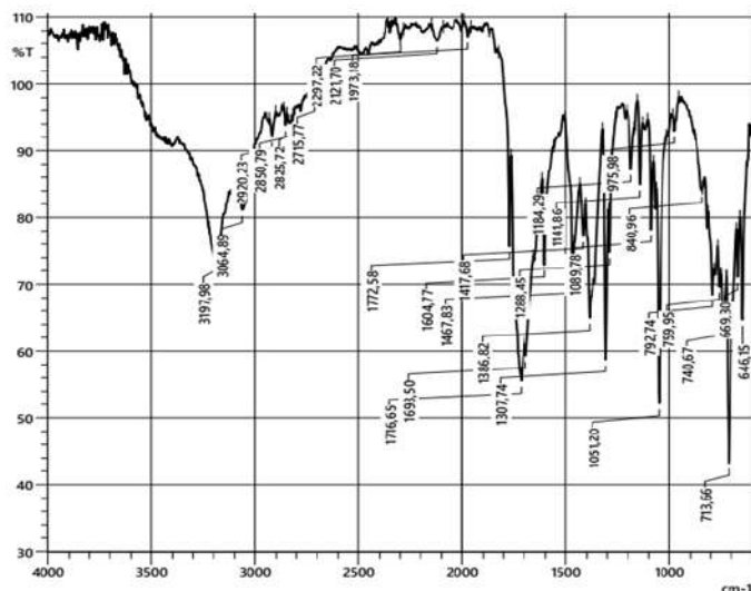
1-rasm. Rux xlorid asosidagi rux ftalotsianin pigmentini IQ spektri
