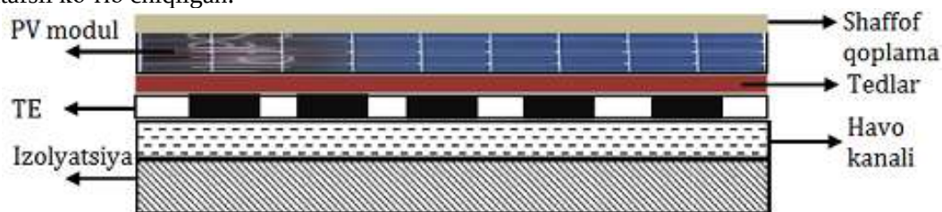
4-rasm. Termoelektrik generatorli PVT tizim
