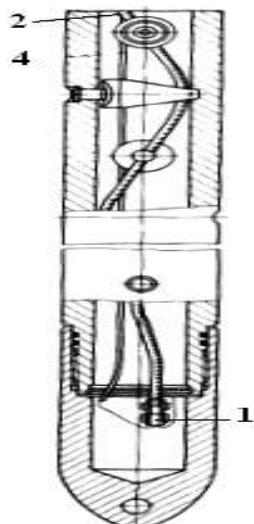
1-rasm. PK105DU korpusli kumulyativ perforatorining qurilmasi:
