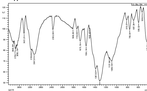
2-rasm. [\text{Cr}_2(\text{Biu})_2(\text{Gln})_2(\text{H}_2\text{O})_2](\text{NO}_3)_2 kompleksi IQ spektri
