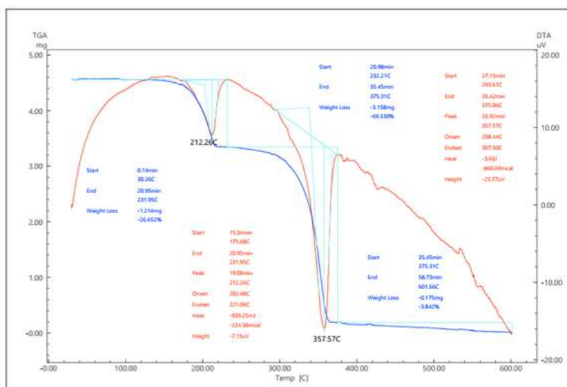
2-rasm. Rux xloridi asosidagi rux ftalotsianinning derivatogrammasi
