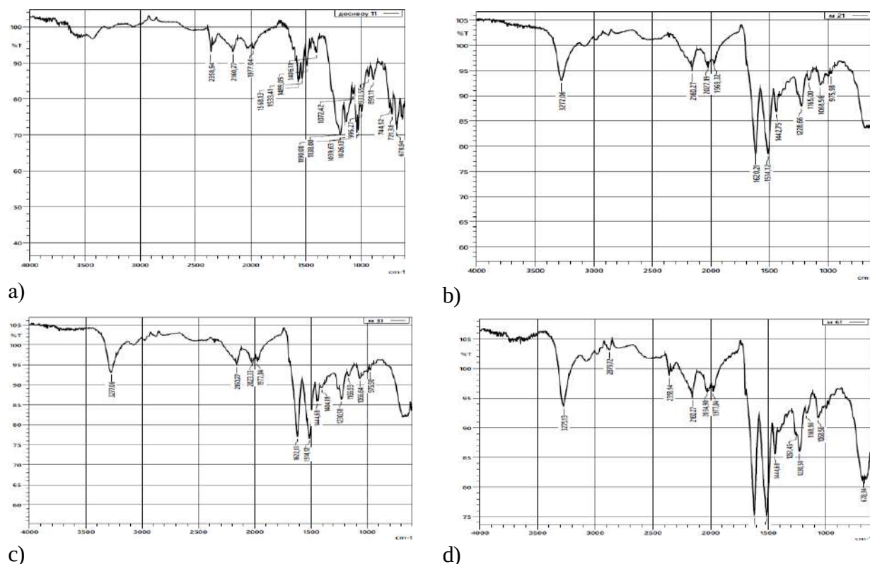
Figure 1. IR Fourier spectra a) dye “Reactive blue K”; b) undyed silk fabric; c) dye-dyed fabric; d) dyed fabric using chitosan.
