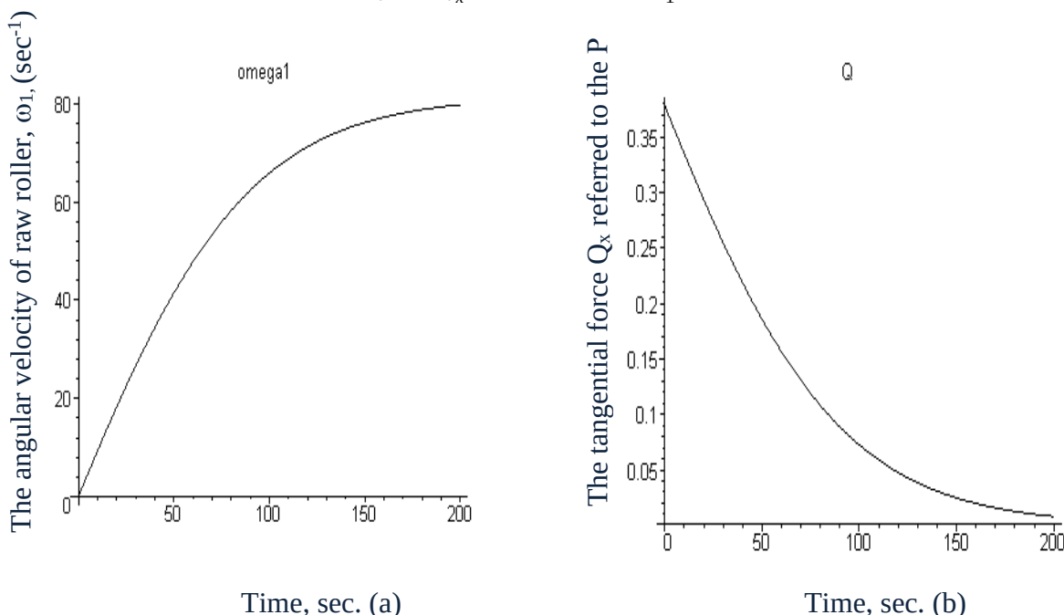
Figure 4. Changing the angular velocity of raw roller \omega_1 (sec -1 ) and tangential forces Q = -Q_x / P in time, at R_1 = 0.16m
