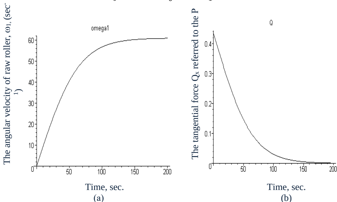
Figure. 3. Changing the angular velocity of raw roller \omega_1 (sec -1 ) and tangential forces Q = -Q_x / P in time, at R_1 = 0.2m
