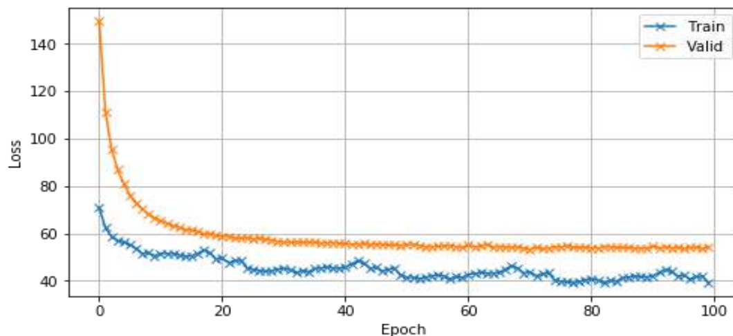
4-rasm. Loss xatoligining o'qitish qadamlarida o'zgarishi
