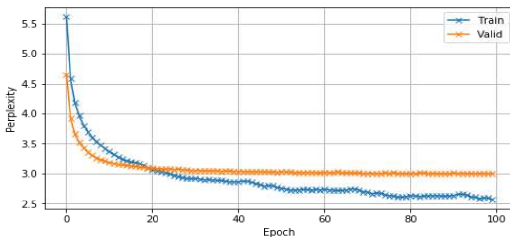
5-rasm. Modelning perplexity ko'rsatkichini o'qitish qadamlarida o'zgarishi.
