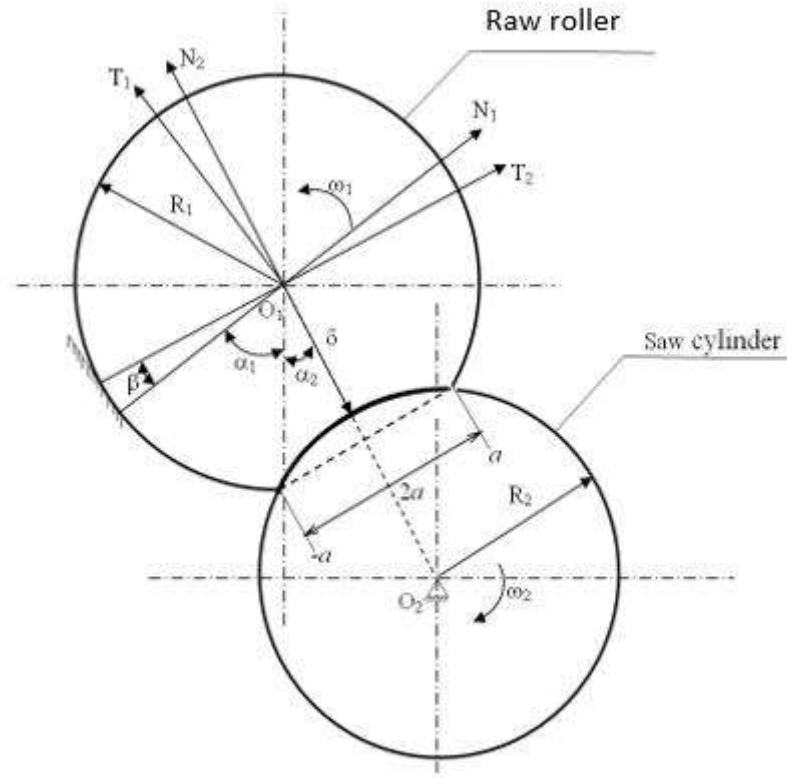
Figure 2. Contact zone of raw roller with the saw cylinder.
