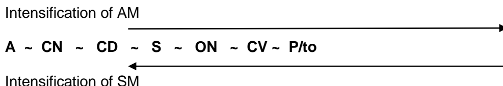
Рис. 3. Graduonimical row of morphological devices according to demarcation of SM and AM***
