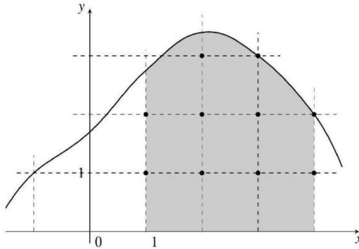
Figure 1. Visual configuration of the bounding manifold f(x) mapping over a discrete two-dimensional integer lattice
