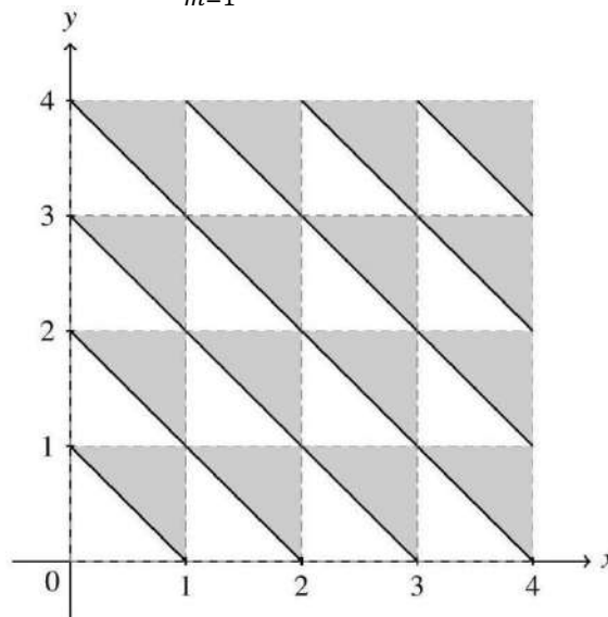
Figure 2. The periodic topological mosaic representation generated by the geometric fractional locus
